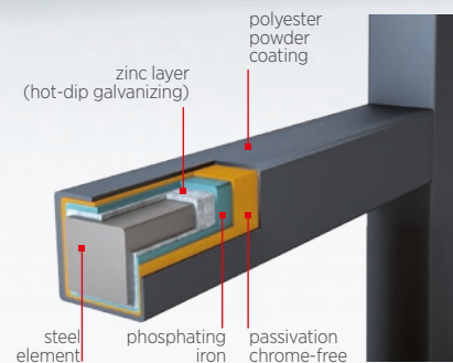
Cross-section of a DUPLEX system secured element
